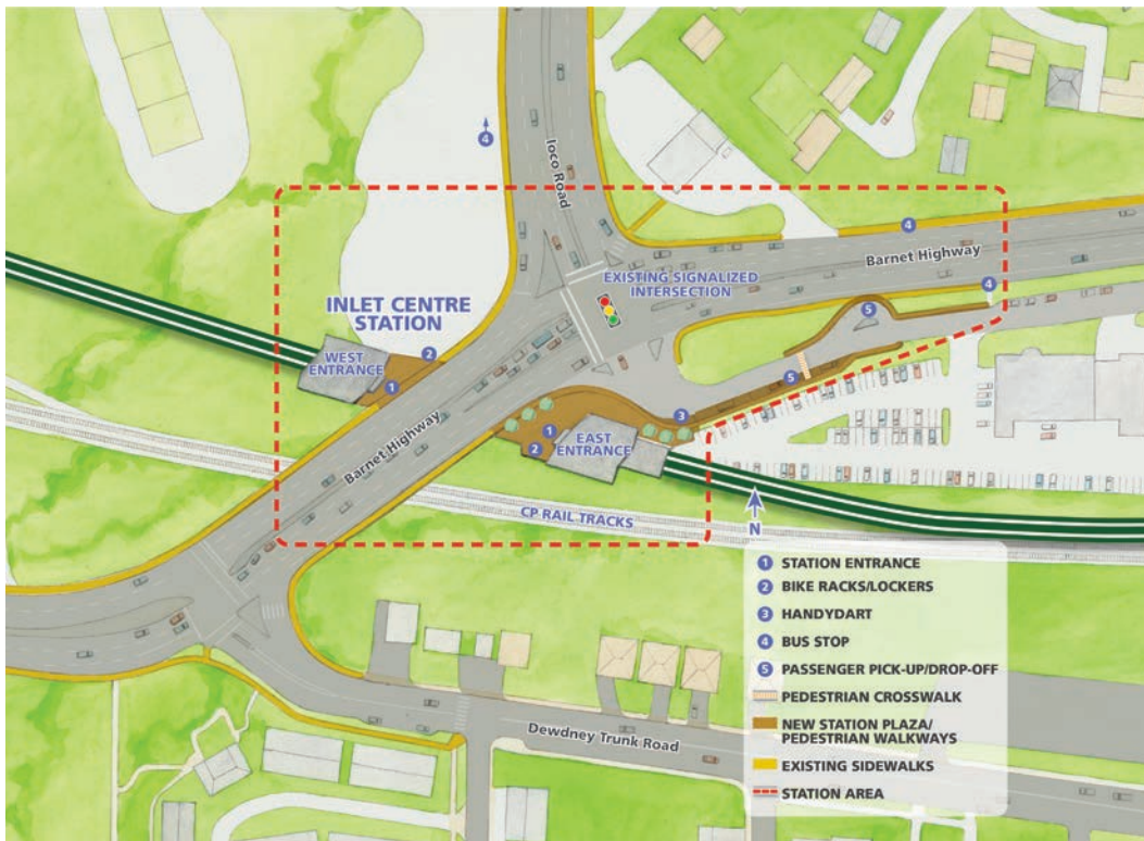
Site context plan for completed Inlet Centre Station
